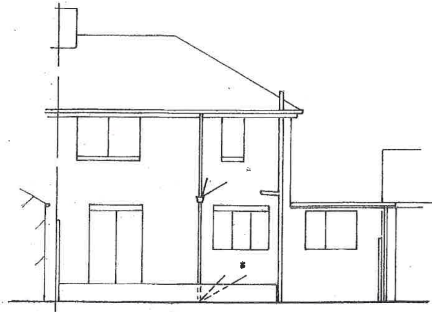
EXISTING REAR 1:100
